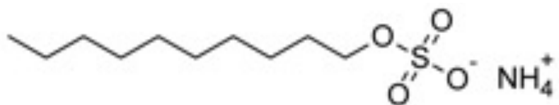
Molecular Structure
